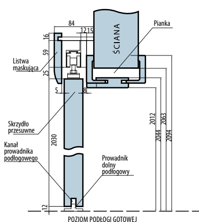
SYSTEM SN 100
